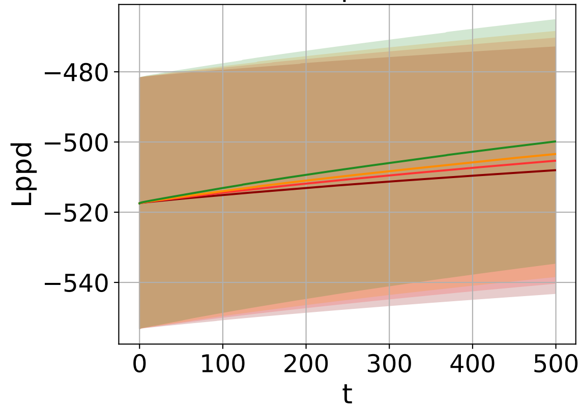
N = 10 particles
