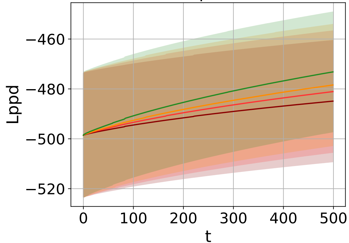
N = 5 particles
